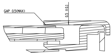
SECTION X1-X1 SCALE 10:1
