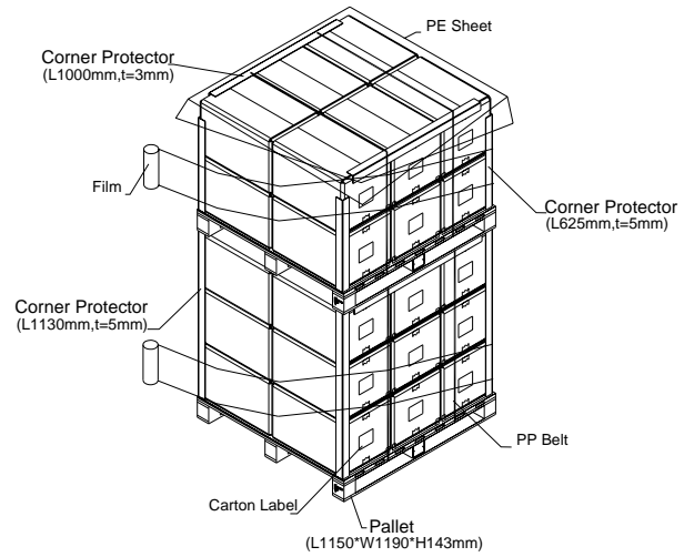
Figure. 8-2 Packing method
